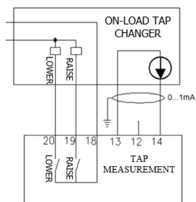
c) Current loop input 0...1 mA
