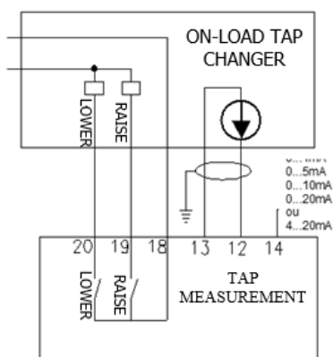
b) Current loop input 0...5 / 0...10 / 0...20 / 4...20 mA
