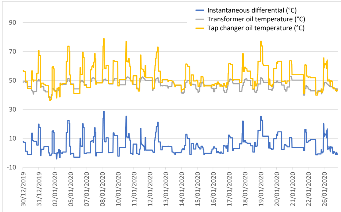
Figure 2 - Temperature measurements of OLTC, transformer and temperature differential
