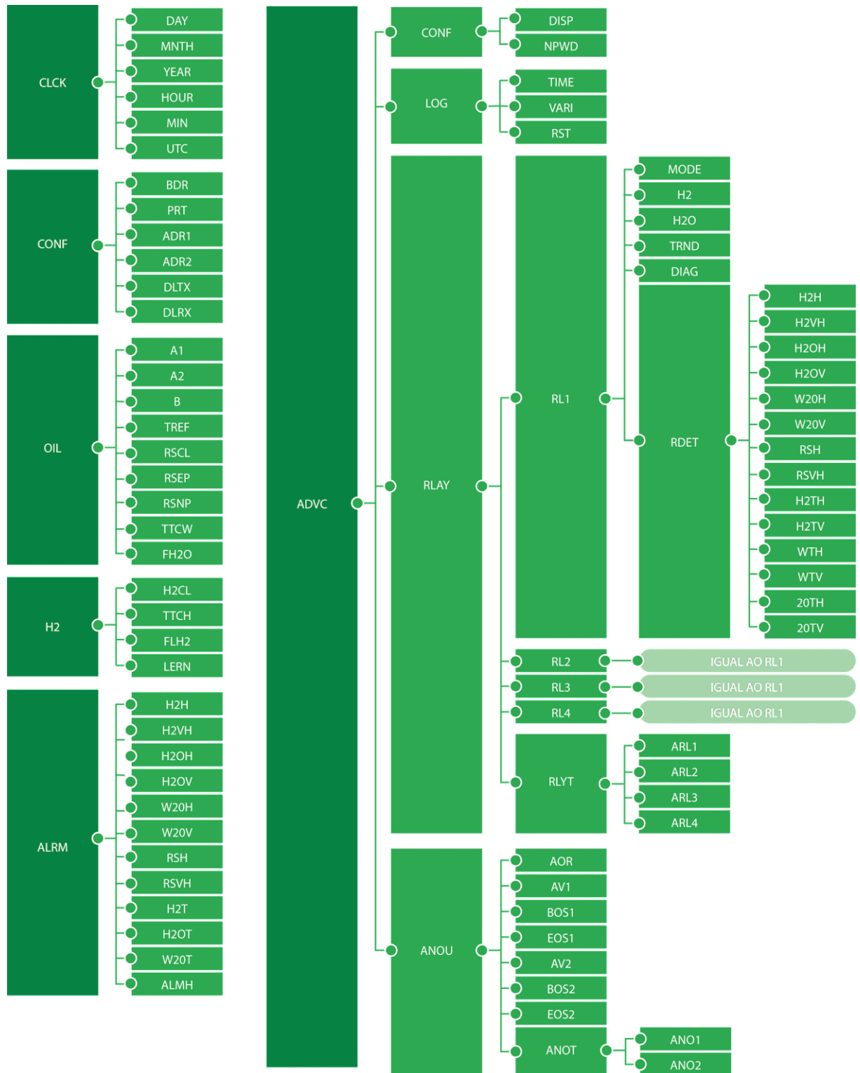
Figure 16 – Structure of menus and submenus
