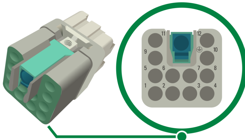
Figure 12 - GMP socket with numbered terminals
