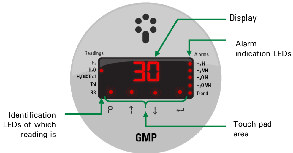
Figure 14 - GMP front display
