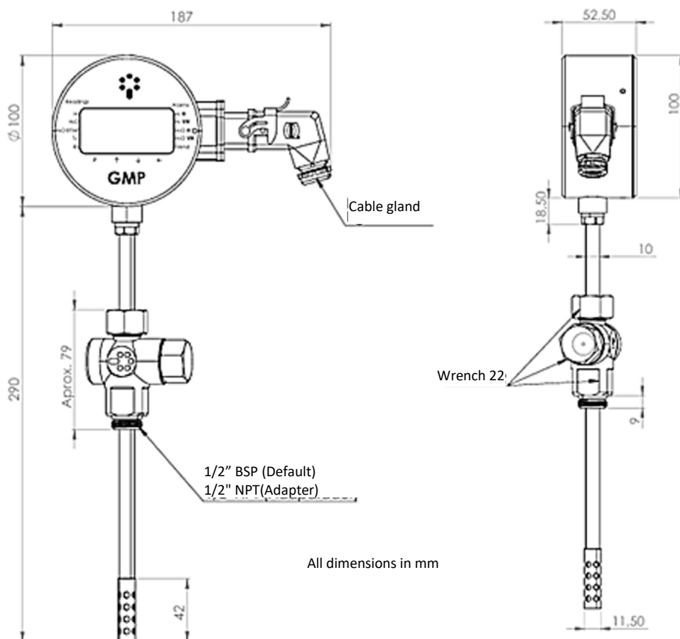
Figure 3 - Equipment dimensions
