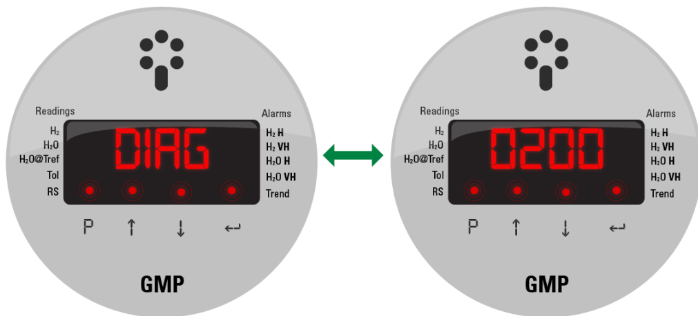
Figure 15 - Self-diagnosis display
