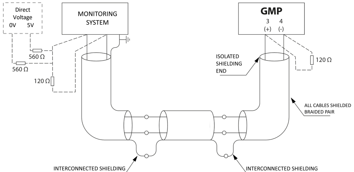
Figure 13 - Connections and grounding in the RS-485 communication network
