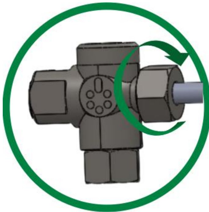
Figure 10 - Tightening the nut on the fastening element
