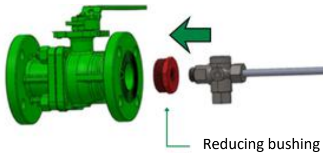
Figure 7 - Fastening element
