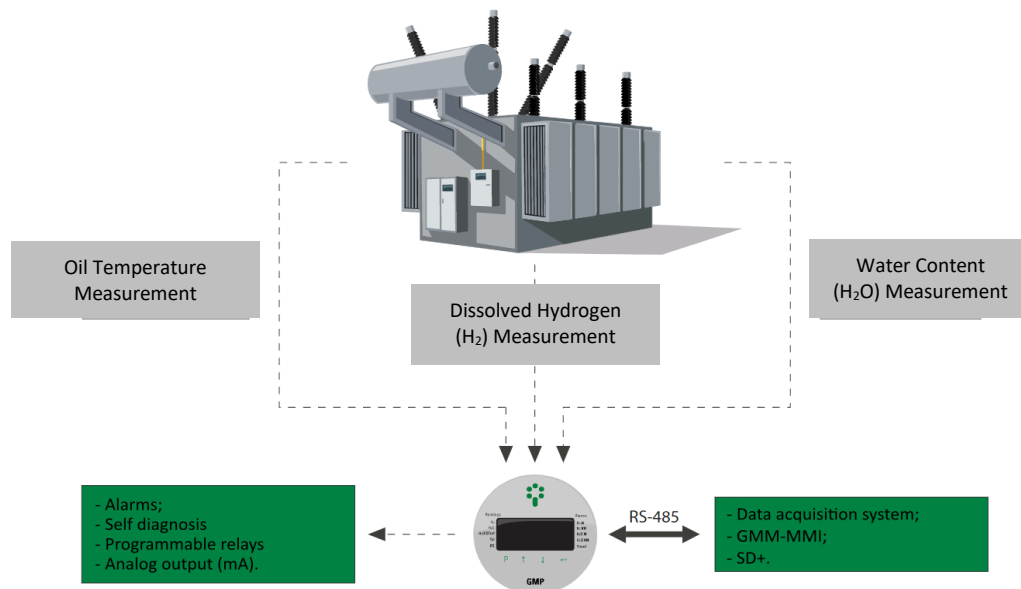
Figure 2 - Composition of the gas and humidity monitoring system
