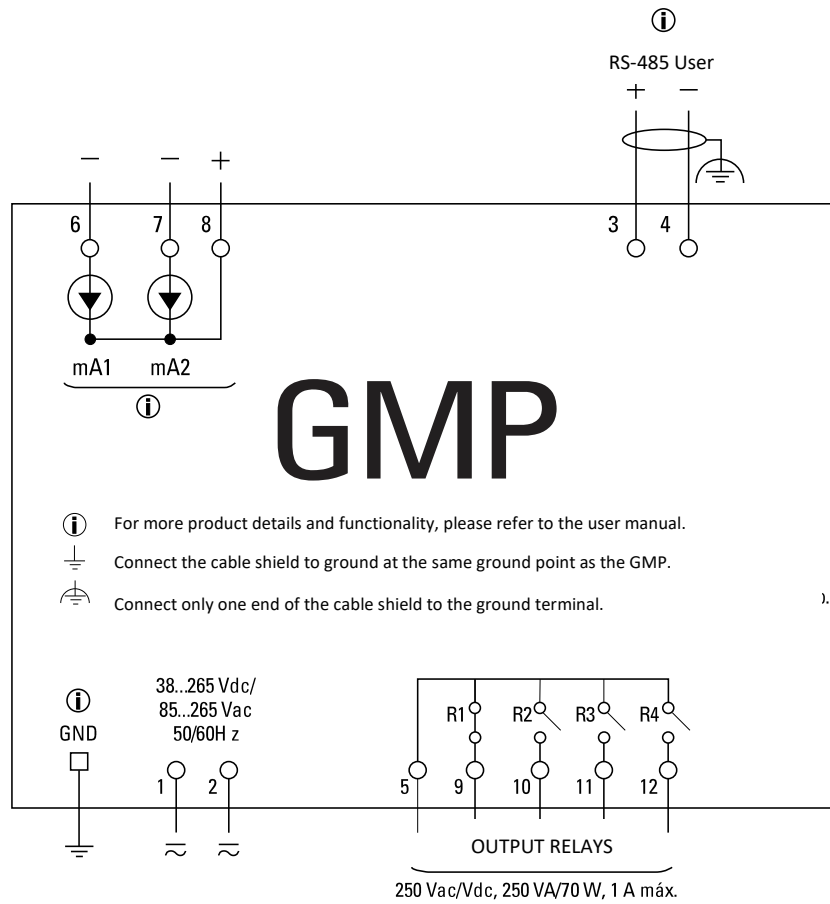
Figure 11 - GMP electrical connection diagram
