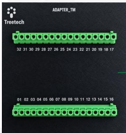
TM1/TM2 Lower Terminal Block
